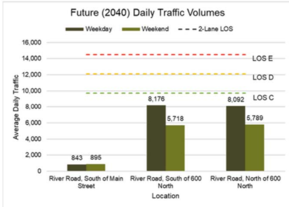
Figure 1: Future (2040) Daily Traffic Volume Projections
